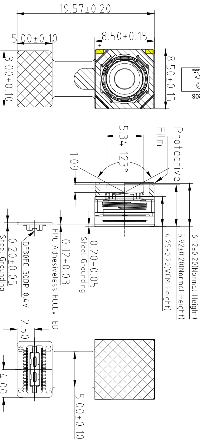
TOP VIEW
